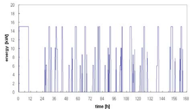
Fig. 5 Energy supplied by boiler
