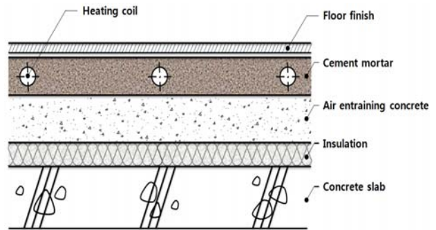
Fig. 2 Section of floor with ondol coil.
