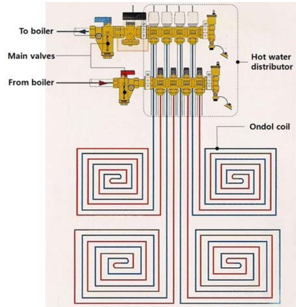
Fig. 3 Ondol coil with hot water distributor.
