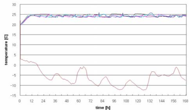
Fig. 6 Indoor and outdoor temperature variations
