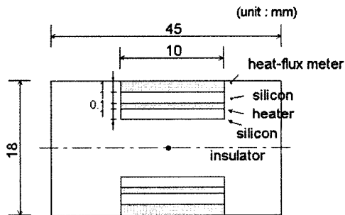
Fig. 8 Calibration device for heat-flux meter.
