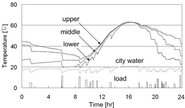
(c) Temperatures in storage tank
