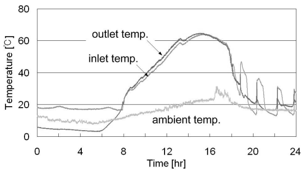
(b) Inlet and outlet temperatures of collector
