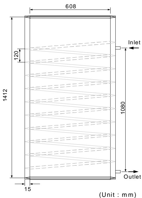
Fig. 1 Spiral-jacketed storage tank.
