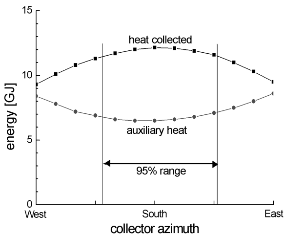
Fig. 4 Acquired and auxiliary heat vs. collector azimuth.
