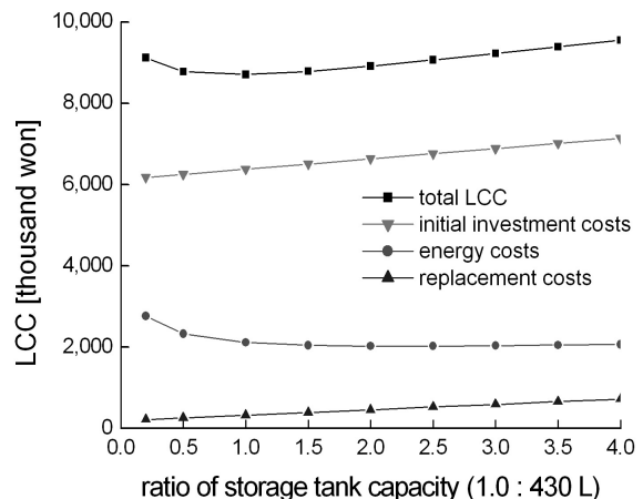
Fig. 9 LCC vs. storage tank capacity.
