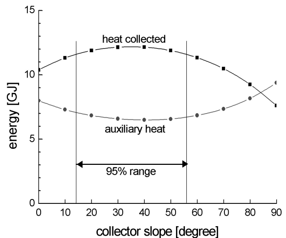
Fig. 3 Acquired and auxiliary heat vs. collector slope.
