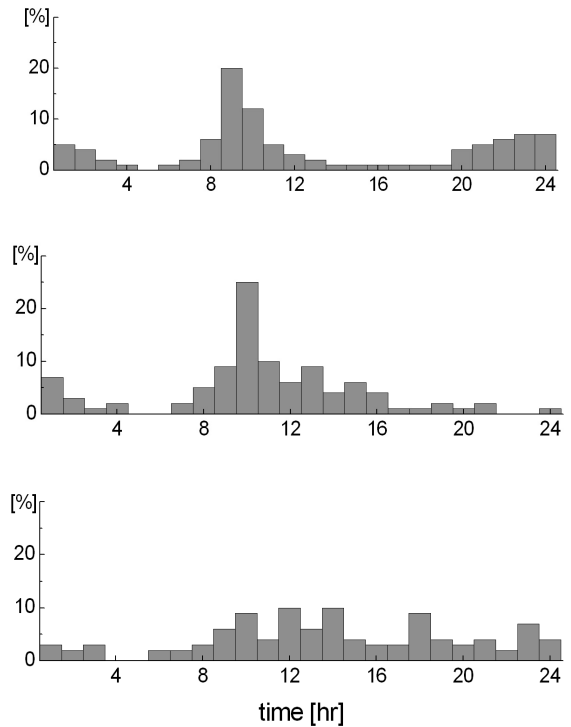
Fig. 2 Load distribution.
