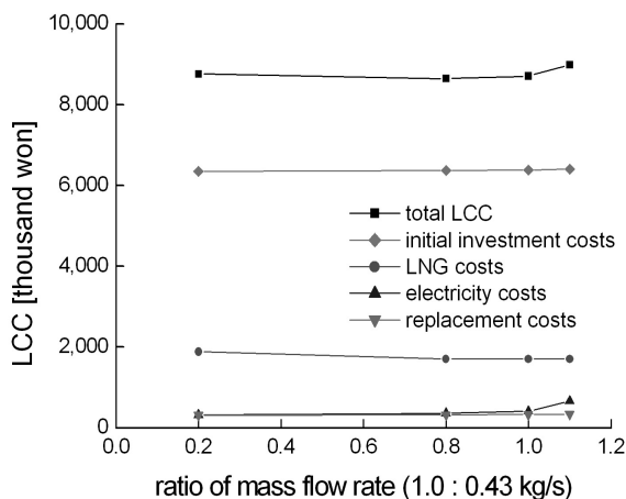
Fig. 10 LCC vs. mass flow rate.
