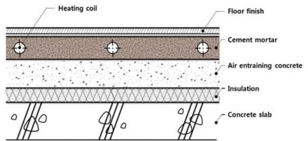
Fig. 2 Section of floor with ondol coil.
