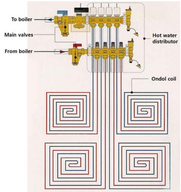
Fig. 1 Ondol coil with hot water distributor.
