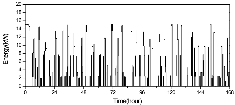
(a) Energy supplied by boiler
