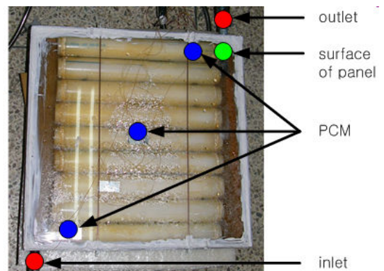
Fig. 2 Location of temperature measurement
