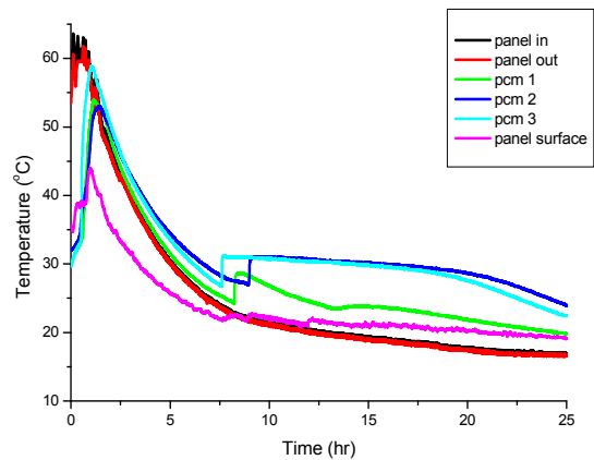
(a) Graph of an experiment by the initial Ondol panel.
