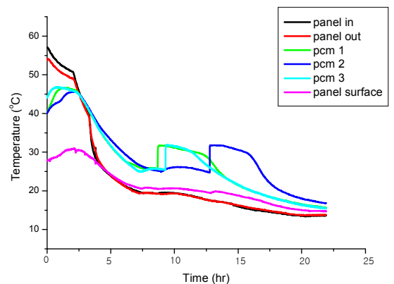
(b) Graph of an experiment by the latter Ondol panel.
