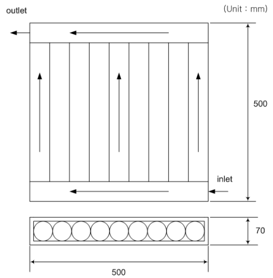
Fig. 1 Schematic of Ondol panel
