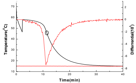
Fig. 3 T-history curve for CH_3COONa \cdot 3H_2O .
