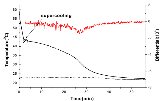
Fig. 5 T-history curve for Lauric acid.
