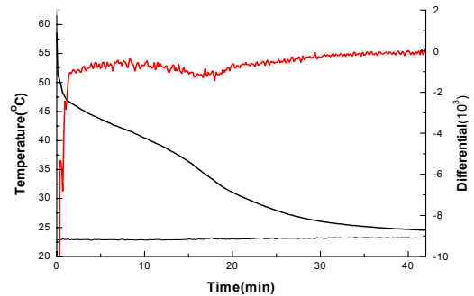
Fig. 4 T-history curve for paraffin.
