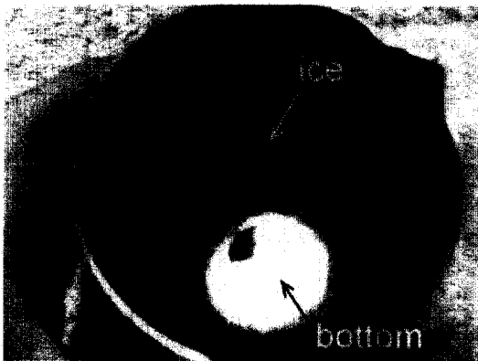
Fig. 5 Ice adhesion on cooling wall (inside wall).
