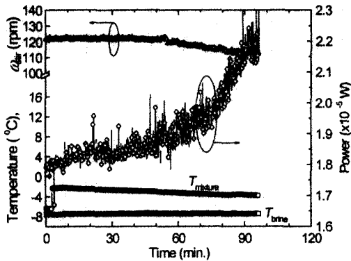
Fig. 9 Time history of temperature and power to an aqueous solution (EG 4 vol%, \Delta T_{\infty} = 4 K).
