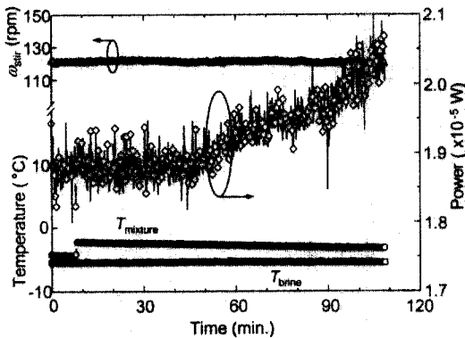
Fig. 3 Time history of temperature and power to an aqueous solution (EG 4 vol%, \Delta T_{sc} = 2\text{K} ).
