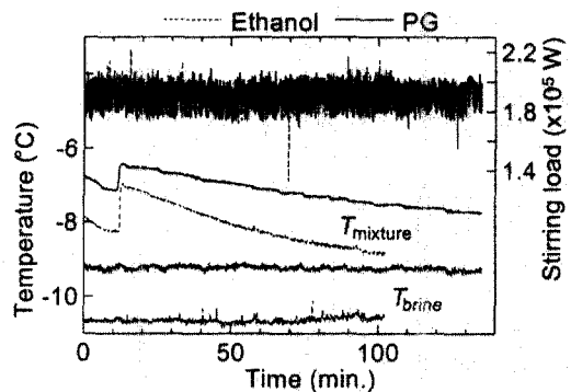
Fig. 11 Time variation of temperature and stirring load to 16 vol% ethanol ( \Delta T_{sc}=1.3 K) or 16 vol% PG ( \Delta T_{sc}=0.7 K) aqueous solution.
