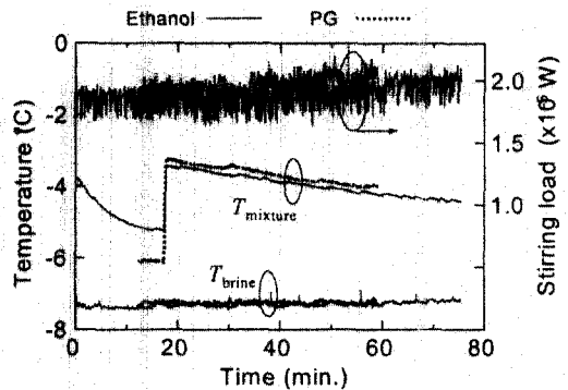
Fig. 10 Time variation of temperature and stirring load to 8 vol% aqueous solution ( (\Delta T_{sc})_{ethanol}=1.8 K, (\Delta T_{sc})_{PG}=2.8 K).
