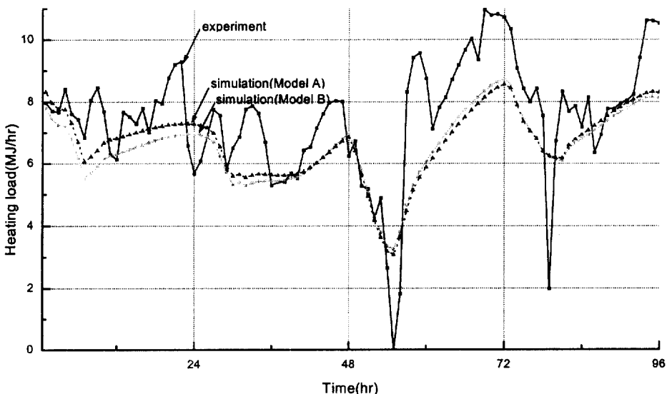
Fig. 4 Comparison of the instantaneous heating load between by the experiment and calculations.
