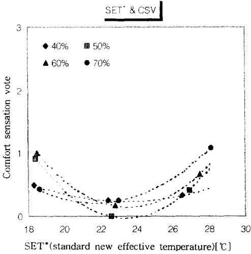
Fig. 12 Relationship of relative humidity and SET*
